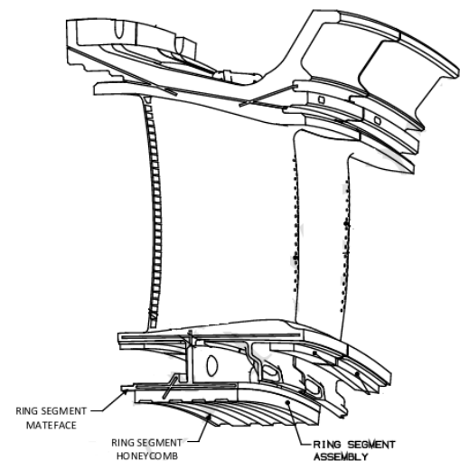
Location of Ring Segment Mateface Weld Repair
